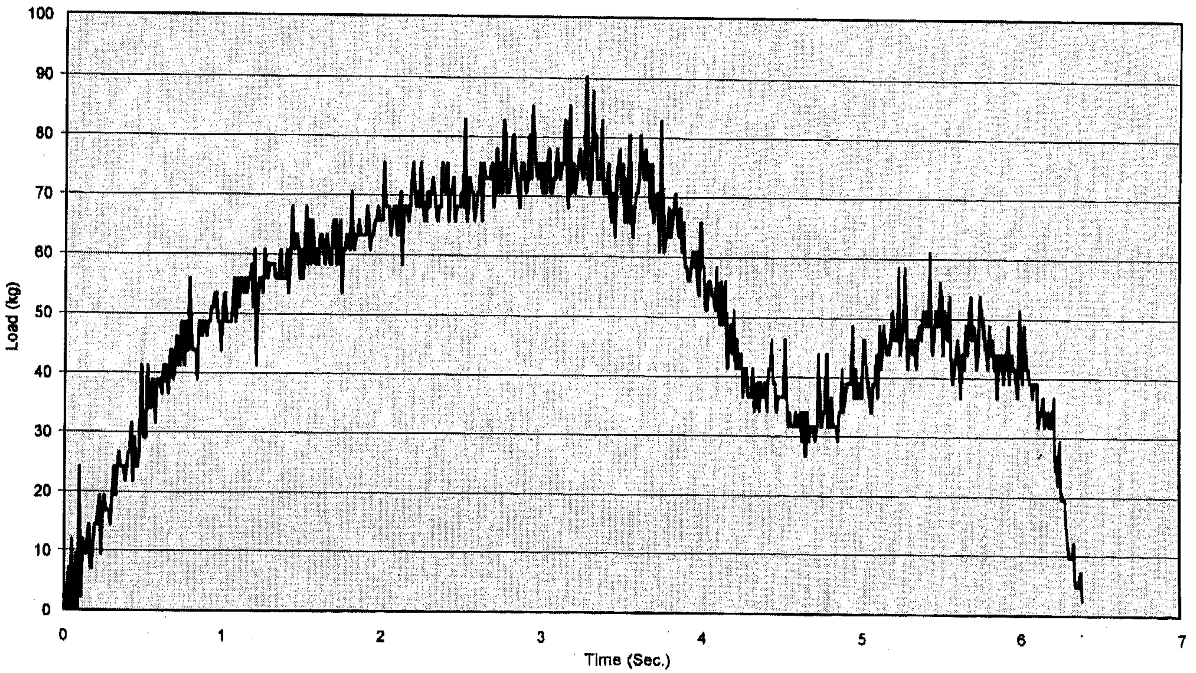
Time-Load Curve (Sample No. 6W4)
